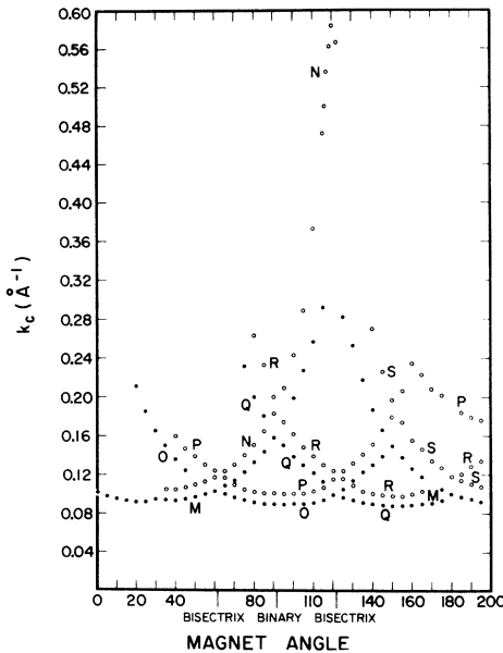
FIG. 4. Caliper values, in \text{\AA}^{-1} , and direction for \vec{n} 7^\circ off the trigonal axis towards the bisectrix axis away from IX.
