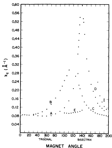
FIG. 3. Caliper values, in \text{\AA}^{-1} , and direction for \hat{n} parallel to binary axis.
