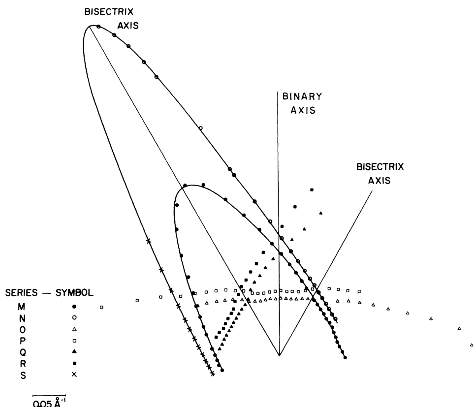
FIG. 8. The electron pocket (series N and S) lying in a plane having \tilde{n} 7^\circ off the trigonal axis towards the bisectrix axis. Series M is the projection of a hole pocket onto this plane. Projections of parts of two other electron pockets (series P and R) and two other hole pockets (O and Q) onto this plane.
