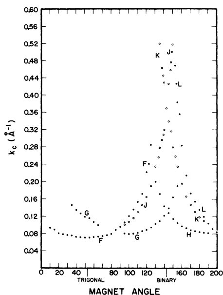
FIG. 2. Caliper values, in \text{\AA}^{-1} , and direction for \hat{n} parallel to bisectrix axis.
