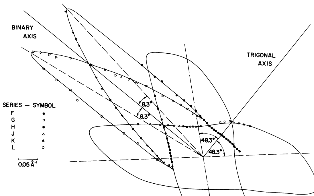
FIG. 6. Projection of two electron pockets (series J , L , F , and K ) and two hole pockets (series G and H ) of Sb onto the bisectrix plane.
